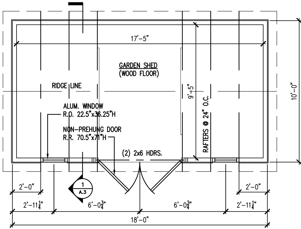
1 A.1 FLOOR PLAN SCALE: 1/4" = 1'-0"
